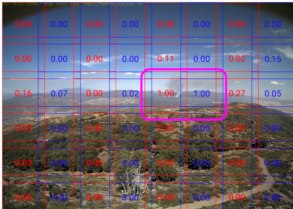
Figure 3. The red and blue grid lines show the overlapping 299 \times 299 squares (two different colors were chosen to make it easier to see the boundaries). The red and blue numbers are the scores returned from the ML inference engine for those corresponding square segments. The two squares highlighted in purple contain a significant amount of smoke and are the only squares that scored above 0.5.
